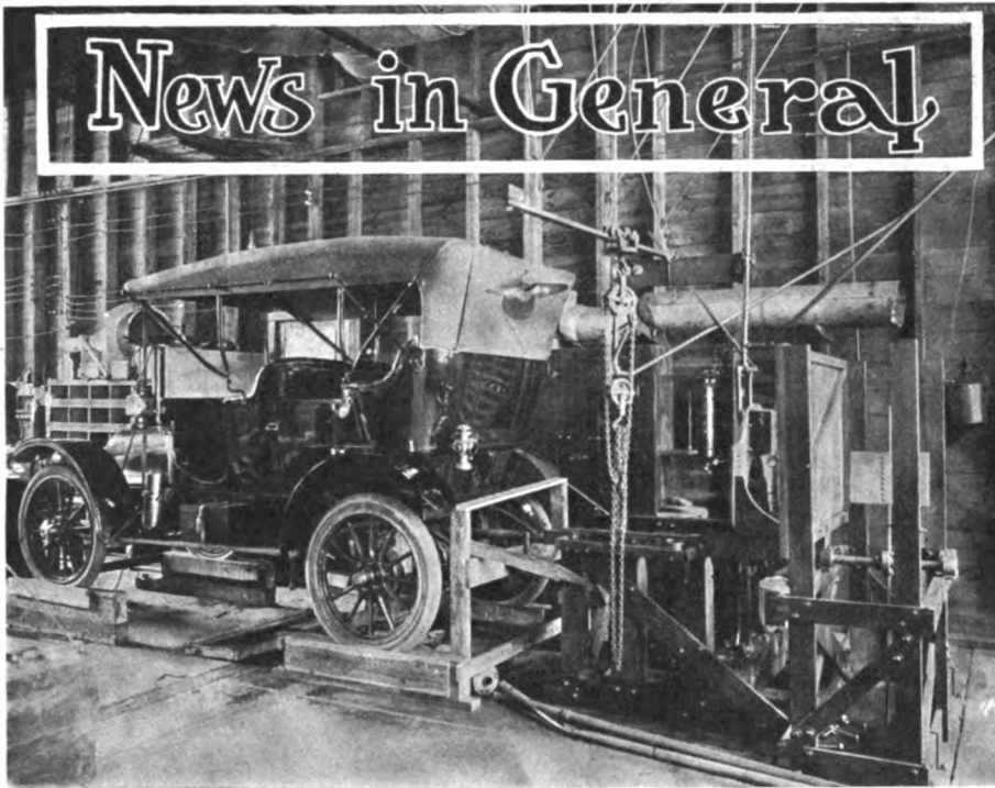
Testing Horsepower of Franklin Engine in Completed Car.
